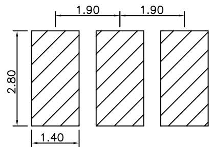
REFERENCE LAND PATTERN
