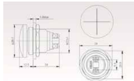
Screw Terminal
